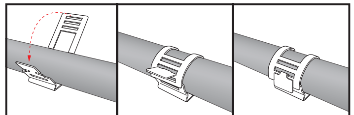
Centralised base fixing, gives a neat appearance to installation
